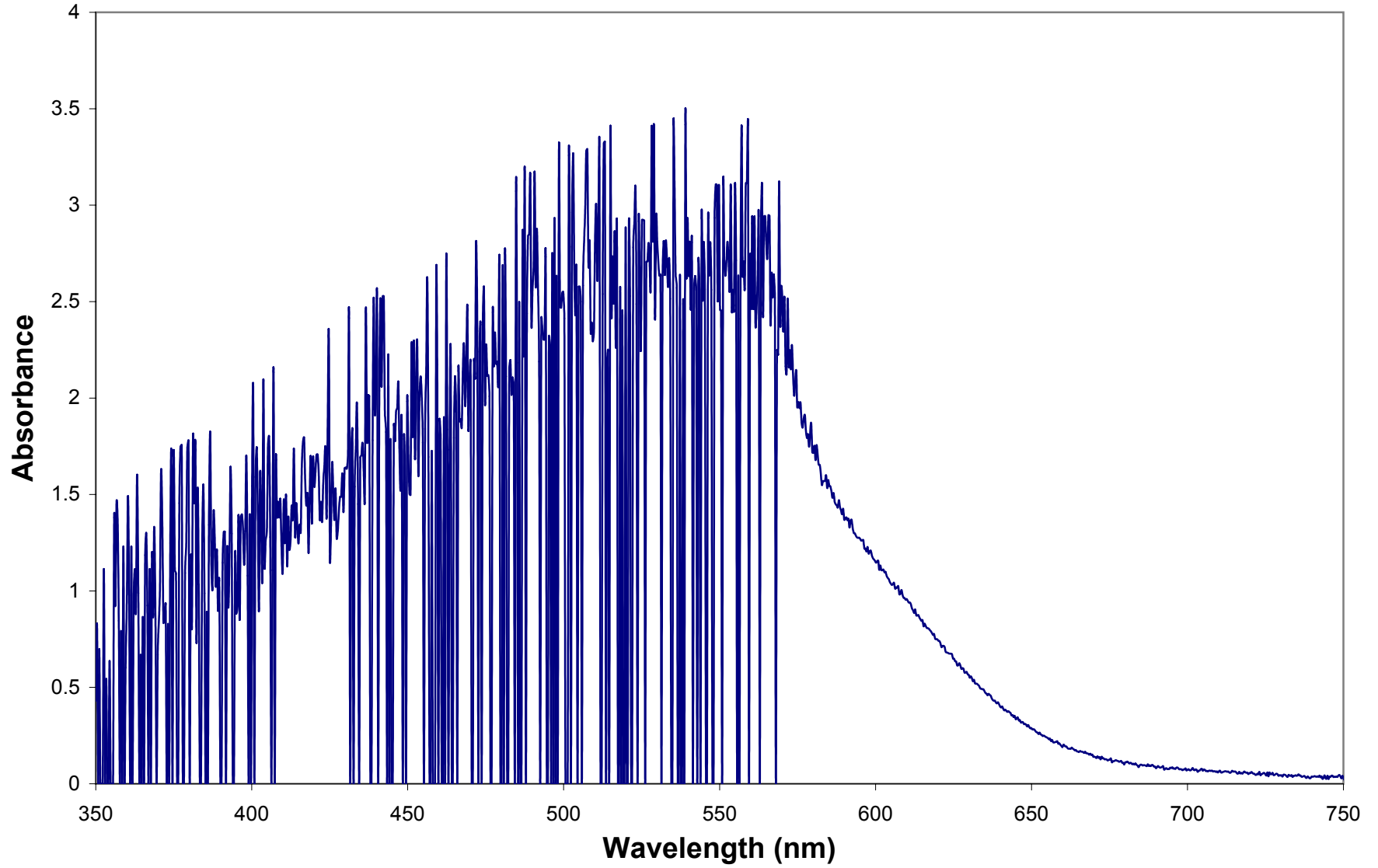
Incandescent Bulb with Red Filter Absorbance Spectrum
